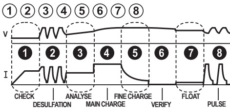
Ladephasen PULSE-TRONIC.
